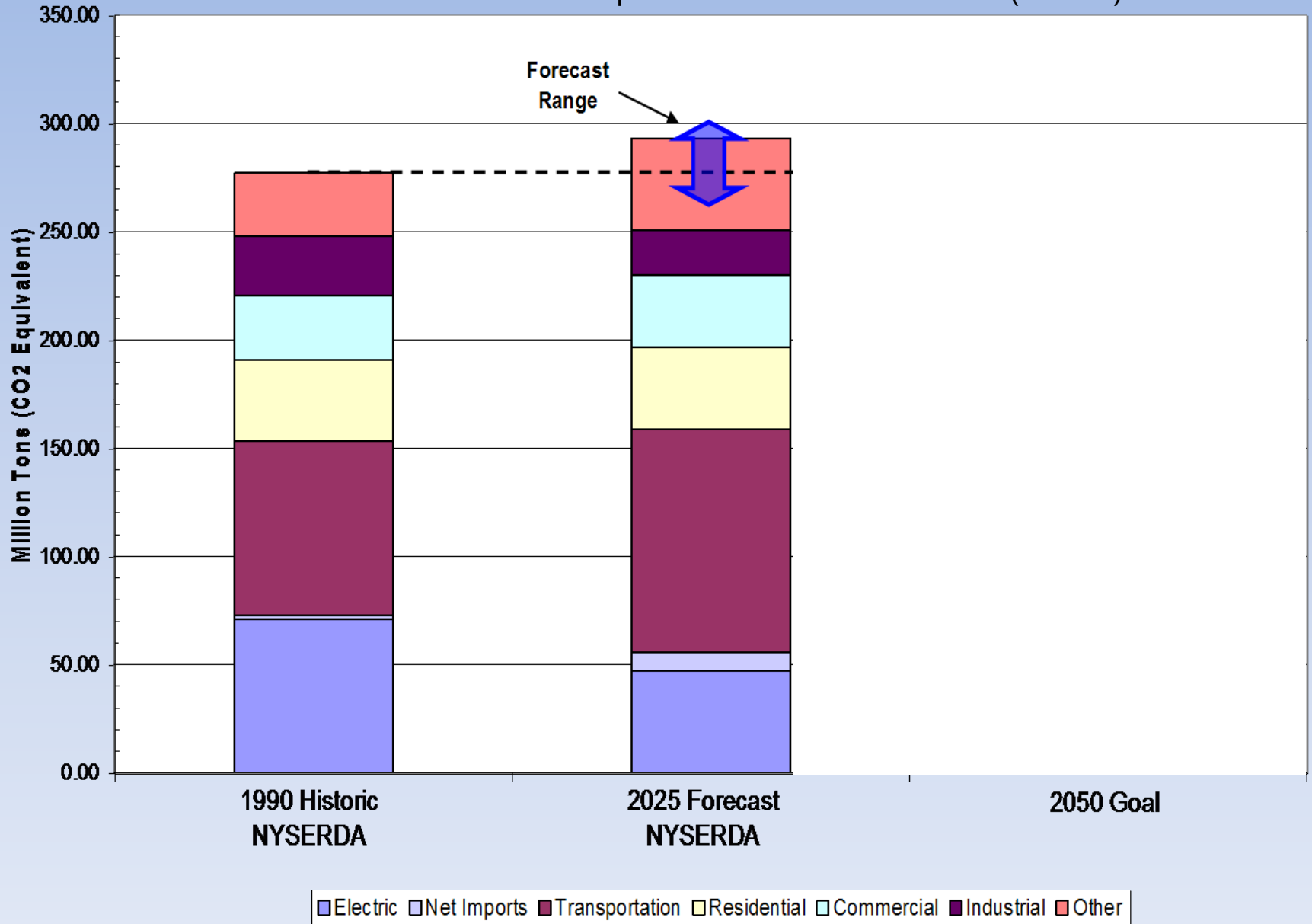
GHG Emission Reductions Required to Meet a 2050 Goal (80X50)
